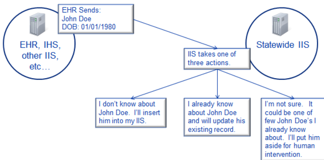
Figure 3.1: Possible Actions Taken When Receiving EHR Data
