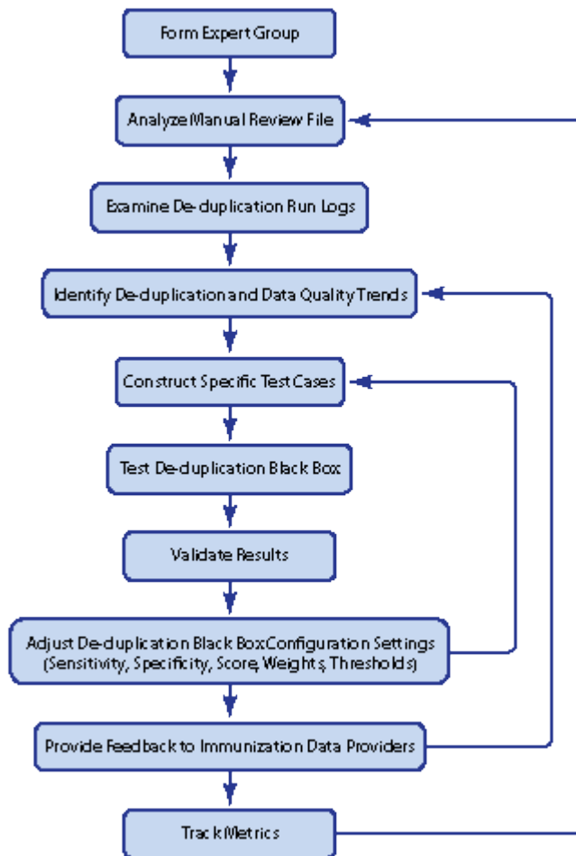
Figure 3.9 Joint Activities Needed For Patient De-duplication Improvement
