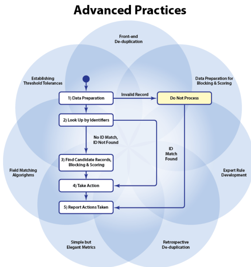
Figure 4: Enhancing the 5 Process Steps through Advanced Practice Techniques
