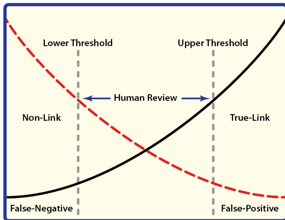
Figure 4.7: Relationship Among Human Review Thresholds and False Negatives and False Positives
