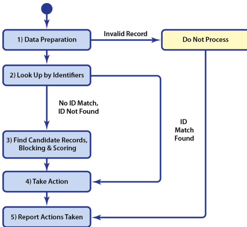
Figure 3.2: Five Major Steps of Typical Patient De-Duplication Process
